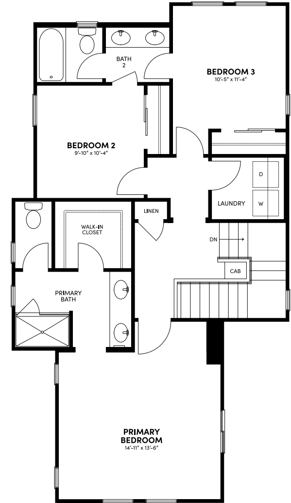
THIRD FLOOR
