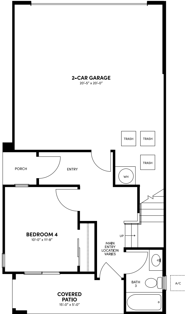
FIRST FLOOR
